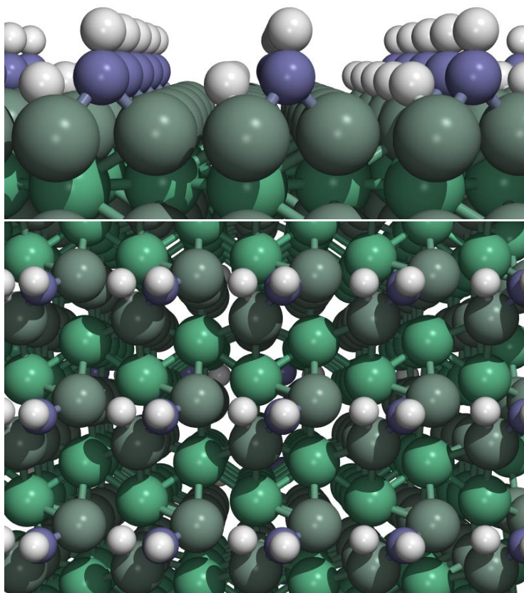
Figure 6.4: TS for methylene decomposition on the Ru(11 \bar{2} 0) surface. Side and top view.
