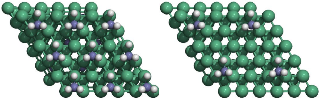
Figure 3.4: Top view of a 2 \times 2 structure and a 3 \times 3 structure.
