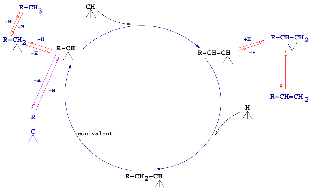
Figure 9.1: Fischer Tropsch, mechanism 1. | indicates atop adsorption, \wedge indicates bridge adsorption, \wedge\wedge indicates three-fold site (fcc or hcp) adsorption and \vee indicates di- \sigma adsorption mode. The R is H for the first cycle and CH_3 for the second one.
