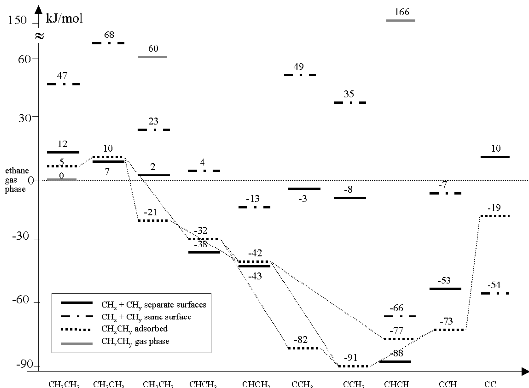
Figure 5.1: Adsorption energies of C_2H_z ( z = 6-0 ), (in dashed lines) CH_x + CH_y ( x, y = 3-0 ) with interactions (dashed lines, line-dot-dot style) and without interactions (plain lines) on the Ru(0001) surface, in \text{kJ} \times \text{mol}^{-1} . The reference line is the Ruthenium (0001) bare surface and gas phase ethane. Only the most stable configurations are shown in this diagram.
