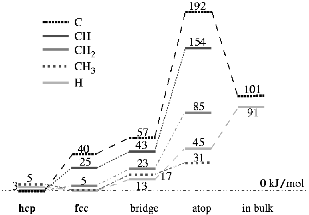
Figure 4.1: Relative energies diagram for \text{CH}_x ( x = 1, 2, 3 ), C and H adsorption on Ru(0001)
