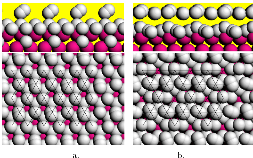
Figure 7.10: H adsorption at 250% coverage: 4 H fcc + 3 H atop + 1 H subsurface + 1 \text{H}_2 (a) and 1 H fcc + 2 H hcp + 2 H bridge + 1 H atop + 2 \text{H}_2 (b). Top and side view.
